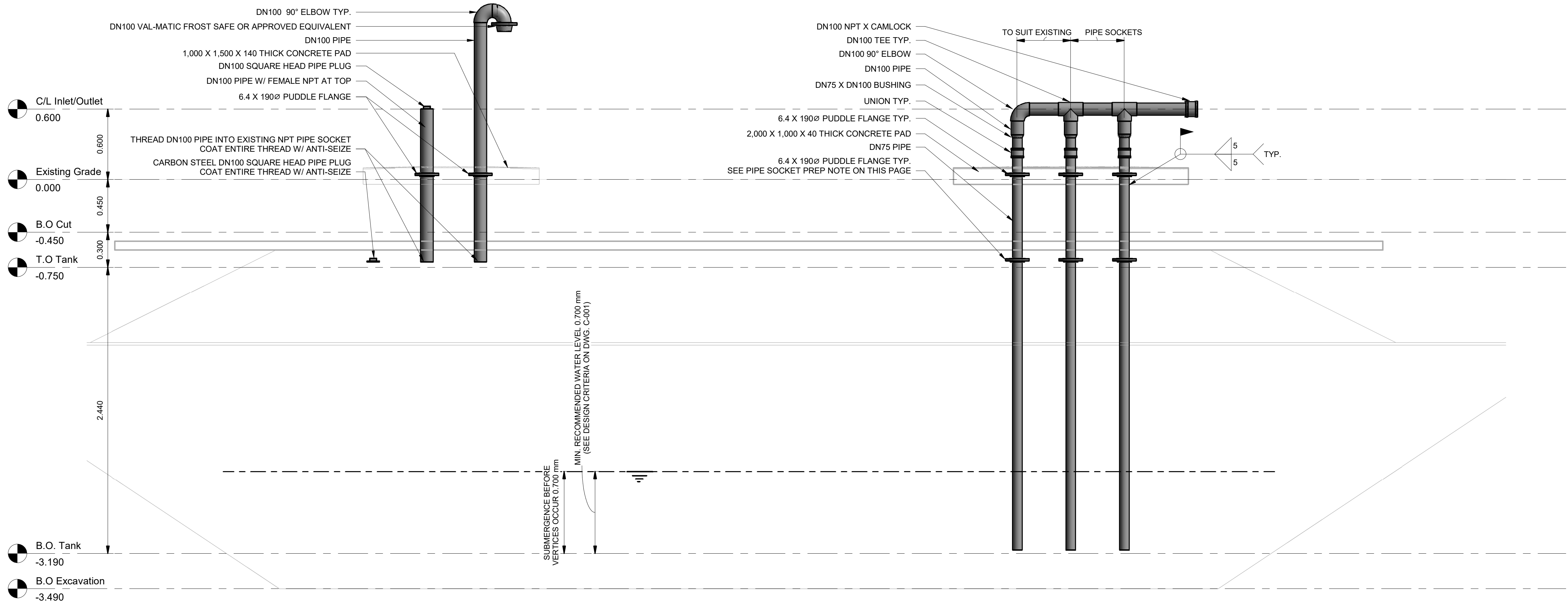
1 Piping Layout 1 : 20
