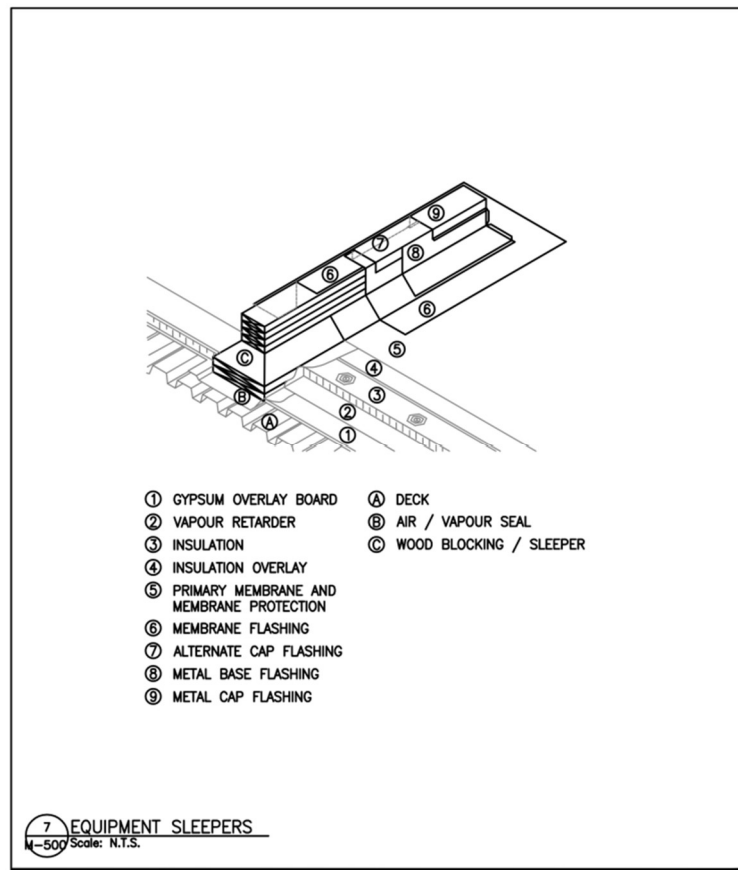
Figure 1. GAHP Sleeper Detail.
